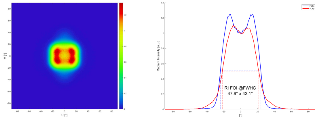
Radiant Intensity Distribution Pattern (Left) and Radiant Intensity Output Profile (Right)
