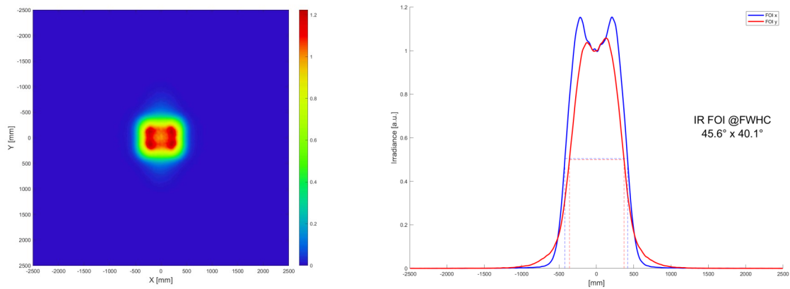
Irradiance Distribution Pattern (Left) and Irradiance Output Profile (Right)
